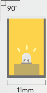
LumiBloc - Straight Edges
